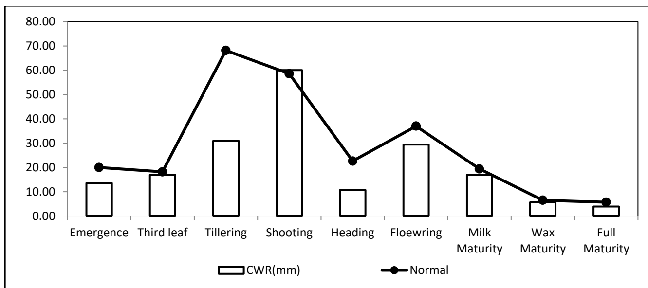
Figure3.11: Crop Water Requirement (CWR) During Crop Life
