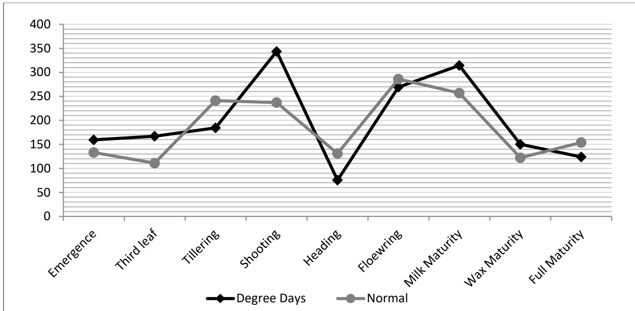
Figure 3.9: Heat units during crop life 2023-24
