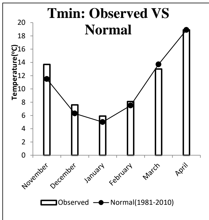
Figure 3.2: Mean Monthly Minimum Temperature (°C) of Faisalabad during the Rabi Season
