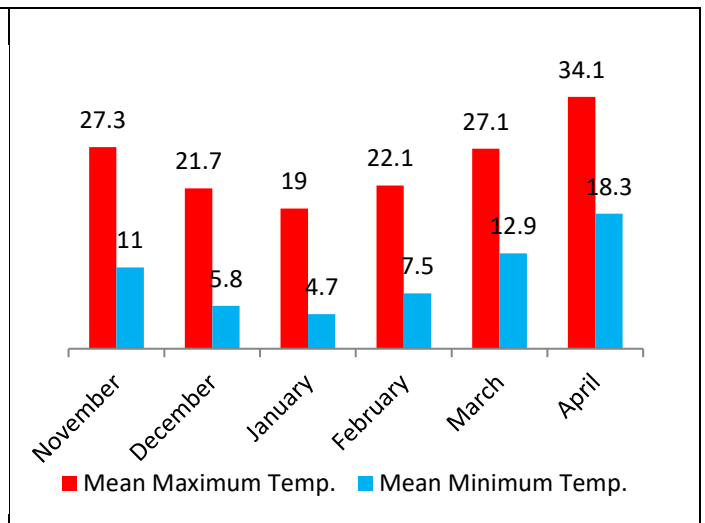
Figure 1.3: Normal (1981-2010) Mean daily Maximum and Minimum Temperature (°C) of Faisalabad during Rabi Season
