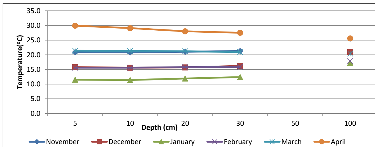
Figure 3.8: Soil temperature during wheat crop 2023-24
