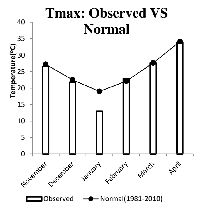
Figure 3.3: Mean Monthly Maximum Temperature (°C) of Faisalabad during the Rabi Season
