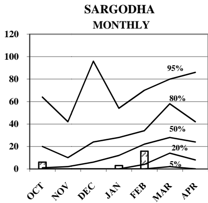
Current Season's Precipitation in mm (Bars) in Comparison to Probabilities of receiving different Amounts (Curves)
