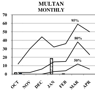
Current Season's Precipitation in mm (Bars) in Comparison to Probabilities of receiving different Amounts (Curves)
