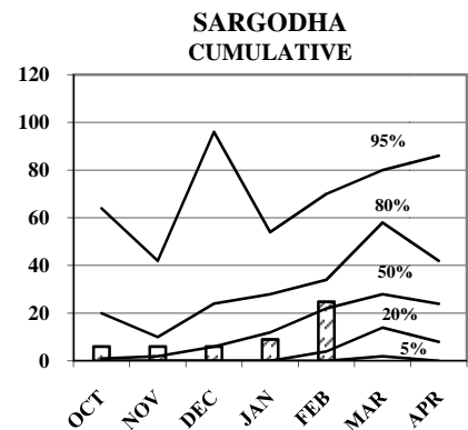
Current Season's Precipitation in mm (Bars) in Comparison to Probabilities of receiving different Amounts (Curves)
