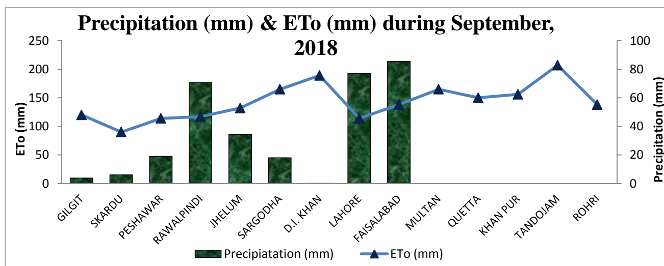
Precipitation (mm) & ETo (mm) during September, 2018 for Major Agricultural plains of the Country
